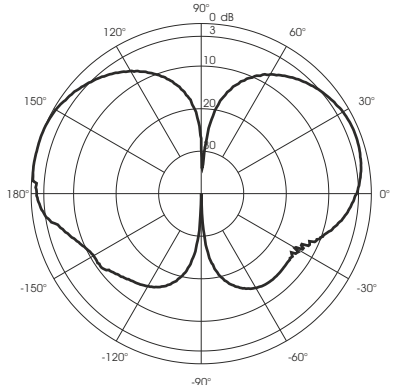
TYPICAL RADIATION PATTERN in E-plane at 158 MHz
