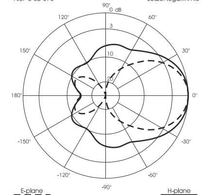
TYPICAL RADIATION PATTERN at mid-band File: E-02-073 Scale: logarithmic
